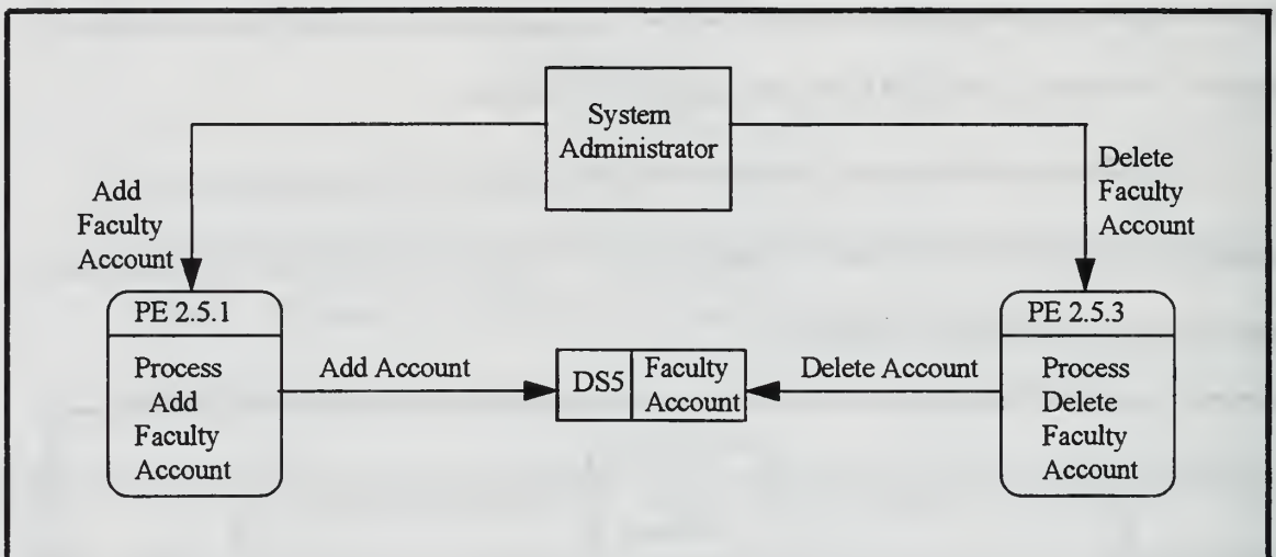
Figure 11. Primitive Level DFD For Maintaining Faculty Account
